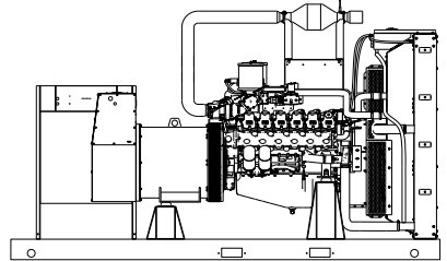
“OPEN” GEN-SET
